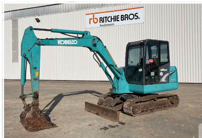
2016 Kobelco SK60-8
