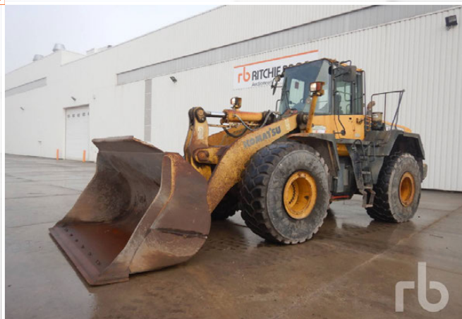
KOMATSU WA470-6
