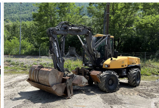
1 / 2 - 2013 & 2012 Mecalac 12 MTX
