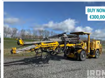
2016 Atlas Copco Boomer 282
