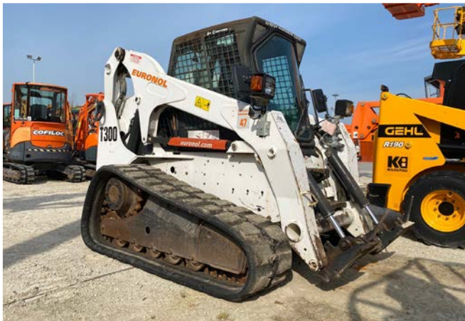
BOBCAT T300HJT
